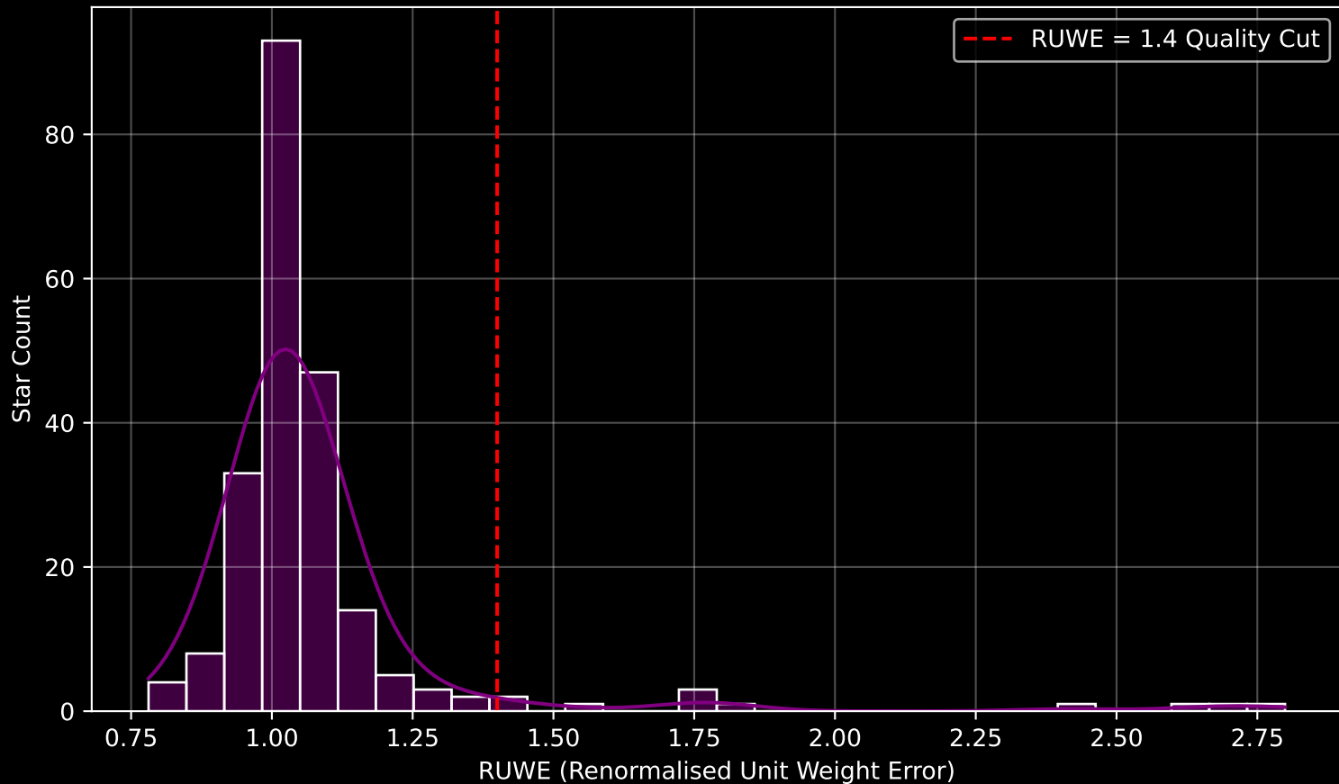
GAPOGEE DR17 Field [109+00] RUWE Distribution (n= 220)
