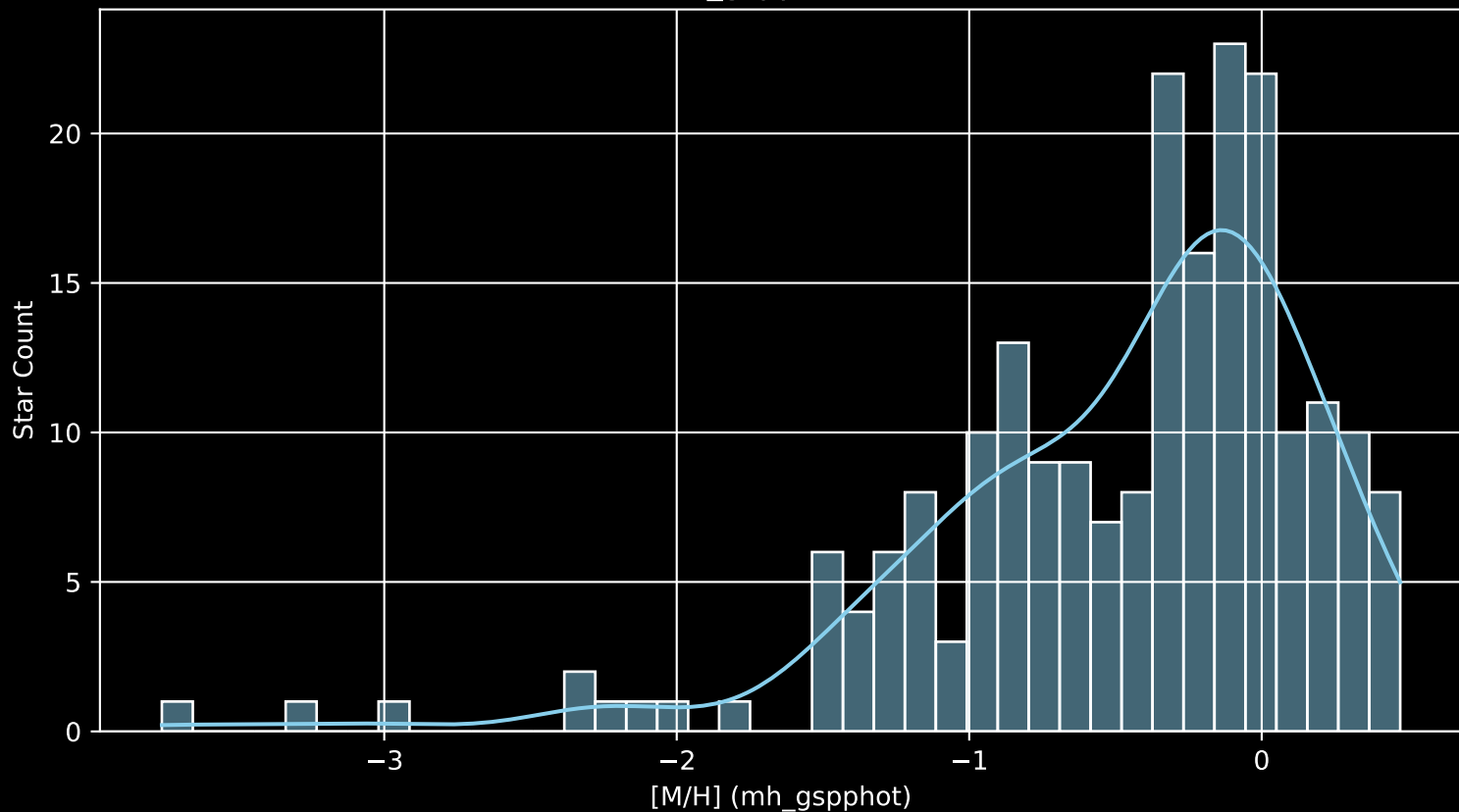
APOGEE DR17 Field: [109+00 [M/H] (mh_gspphot) (n= 214)
