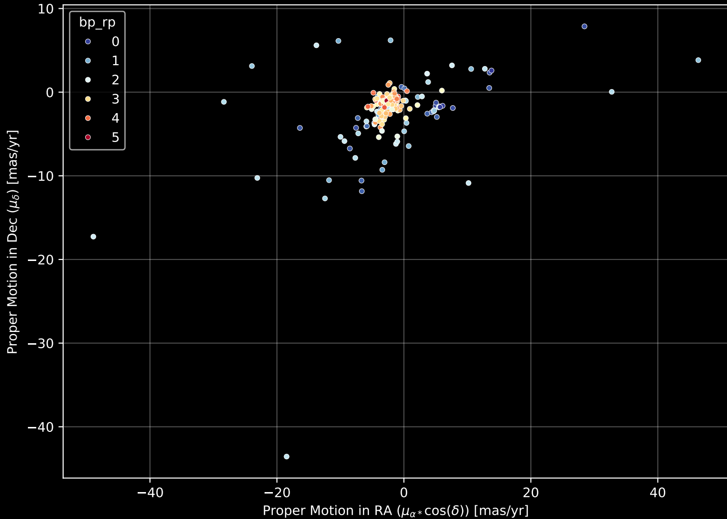
APOGEE DR17 Field: [109+00] Proper Motion Diagram (n= 223)
