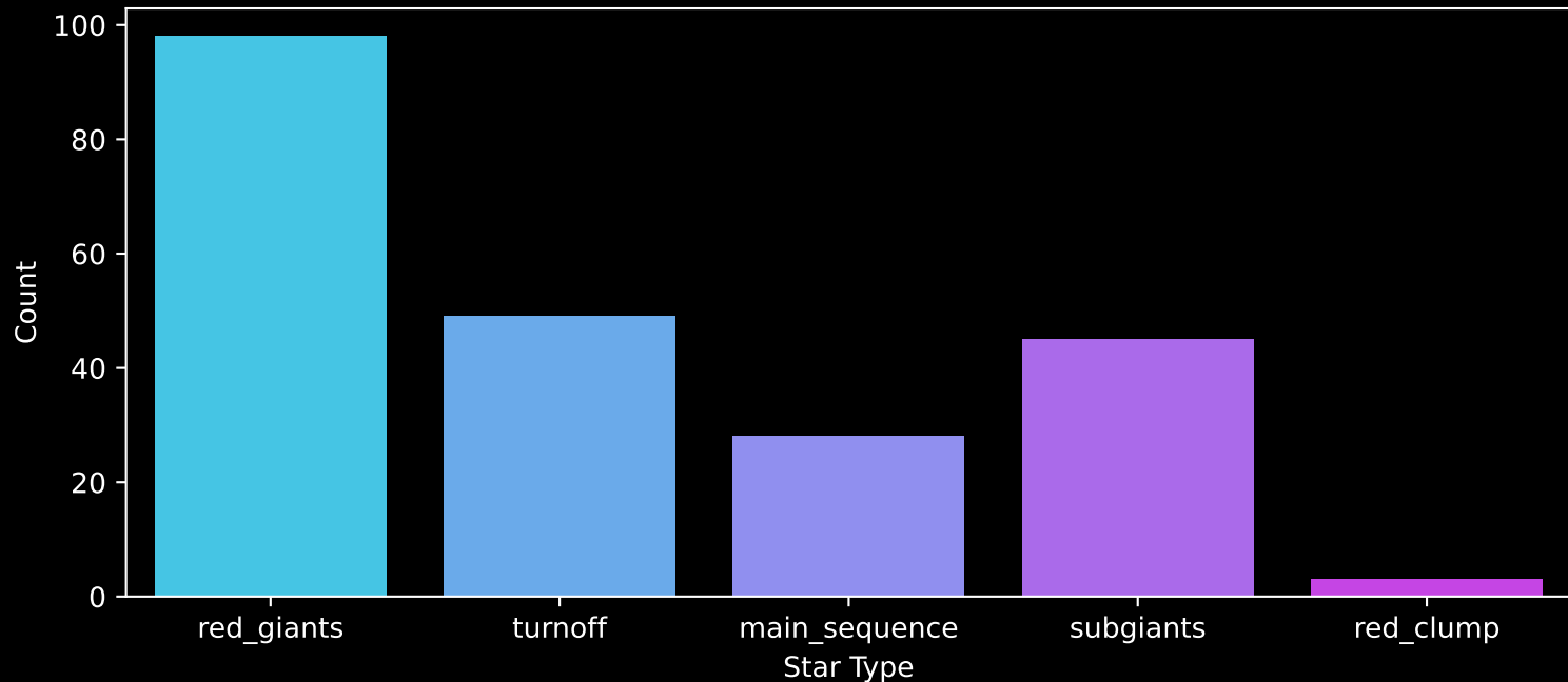
APOGEE DR17 Field: [109+00] Count plot of Star Type
