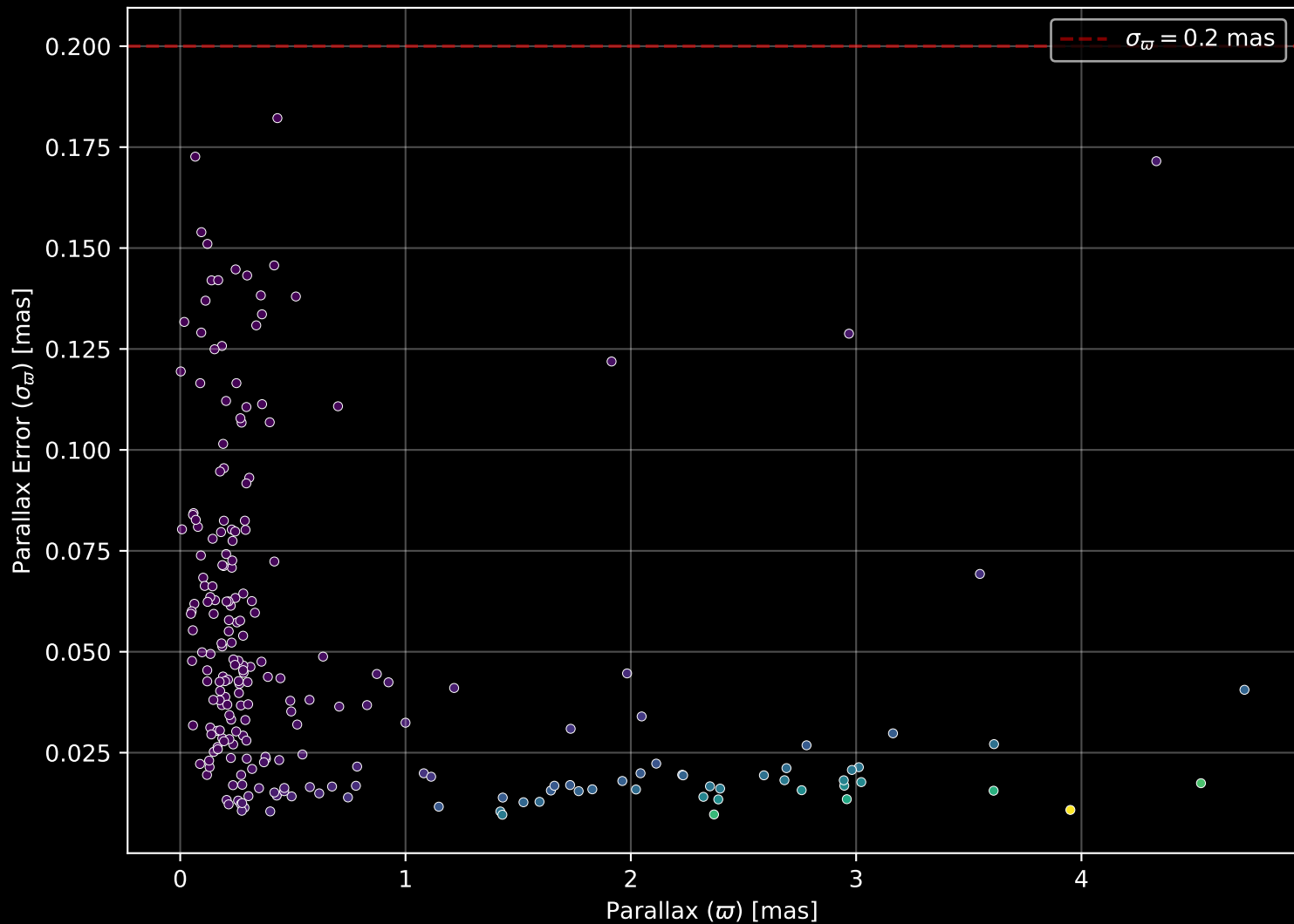
APOGEE DR17 Field: [109+00] Parallax Quality (n= 223)
